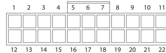
Pin Orientation - Backside of Plug Plug Part No. 2300979-2
