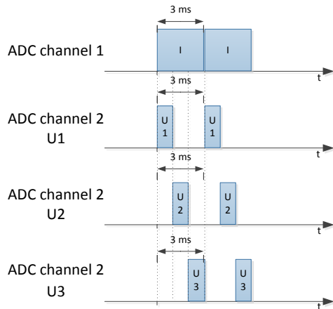
Figure 6 Configuration: 1 current channel, 3 voltage channel, 3 ms measurement interval
