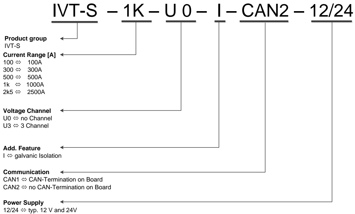
Figure 5: ordering code and part description
