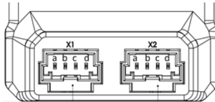
Figure 3: Pin configuration CANbus and power supply
